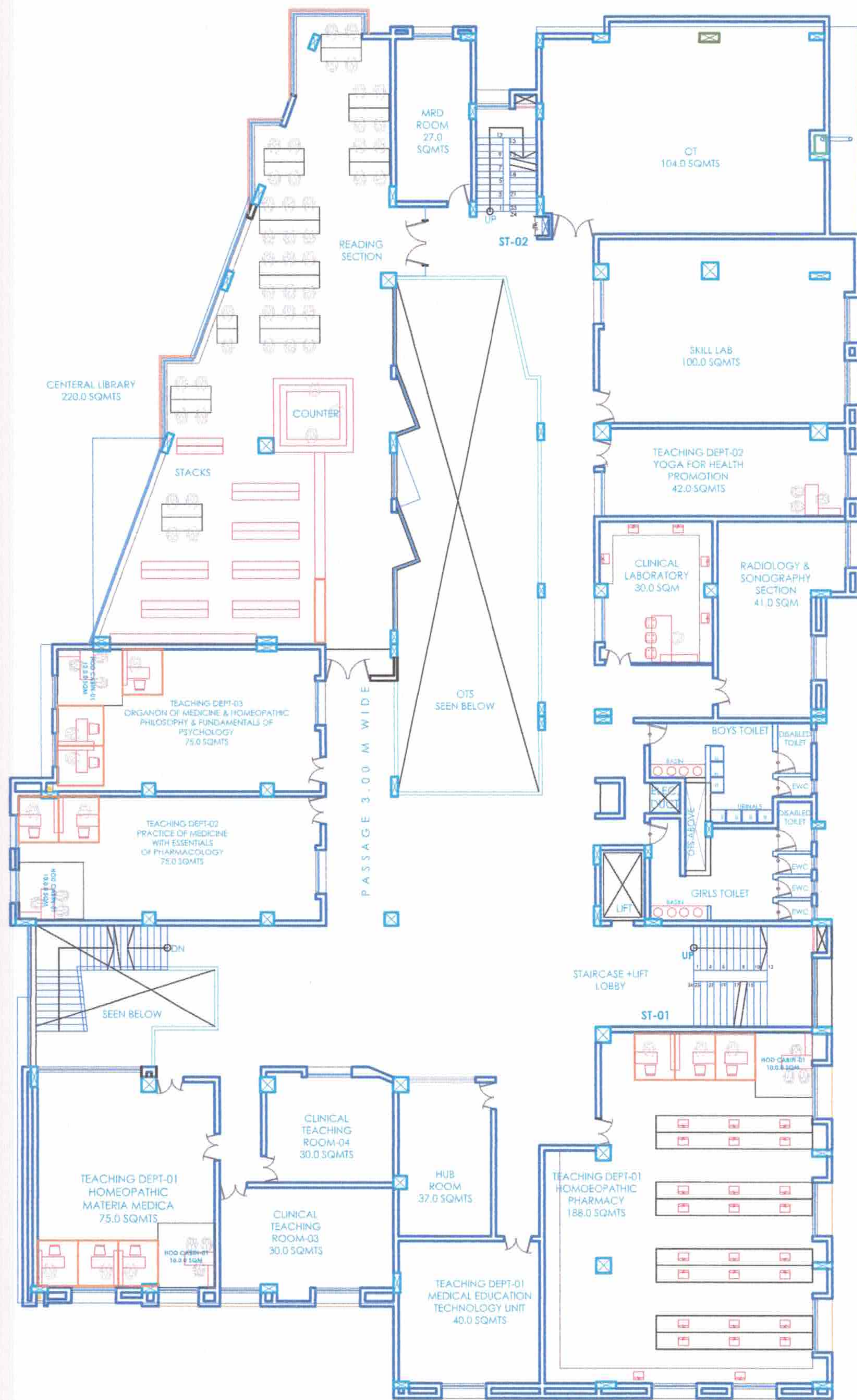
FIRST FLOOR_ FURNITURE ARRANGEMENTS
